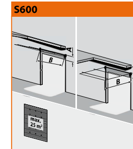
S600 Helix S600 Horizontal track system
