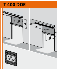
T 400 DDE Springless elevated rail system
