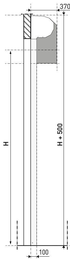
[ Dwarsdoorsnede ]
